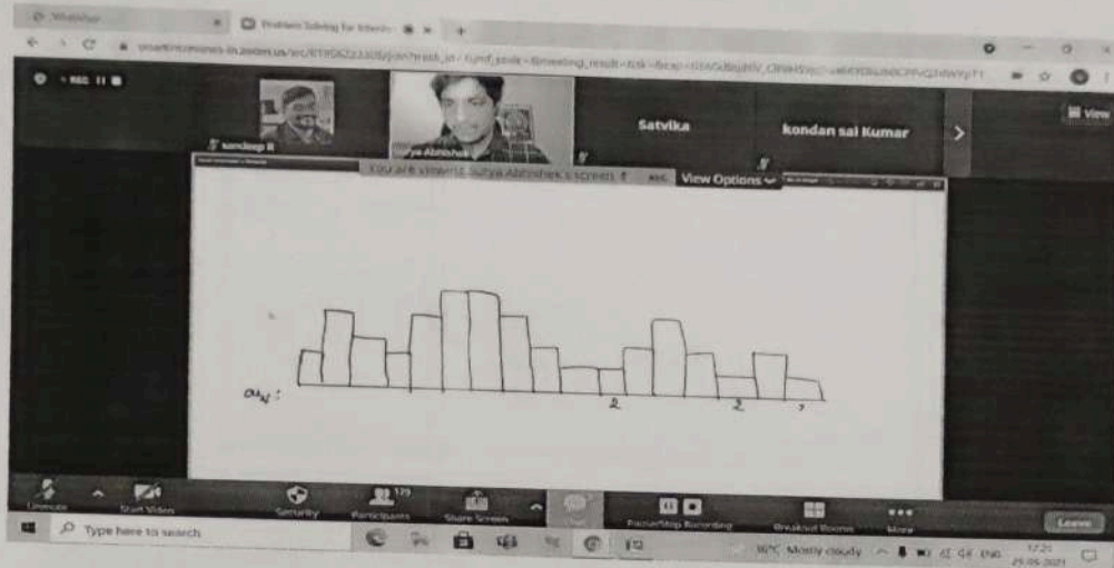
Figure 1 Dynamic Programming
